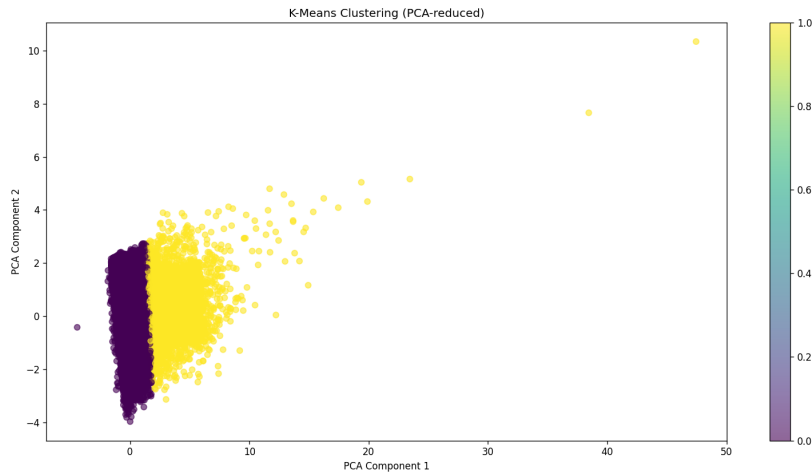
Fig. 11. K-Means cluster visualization (PCA-reduced space)
