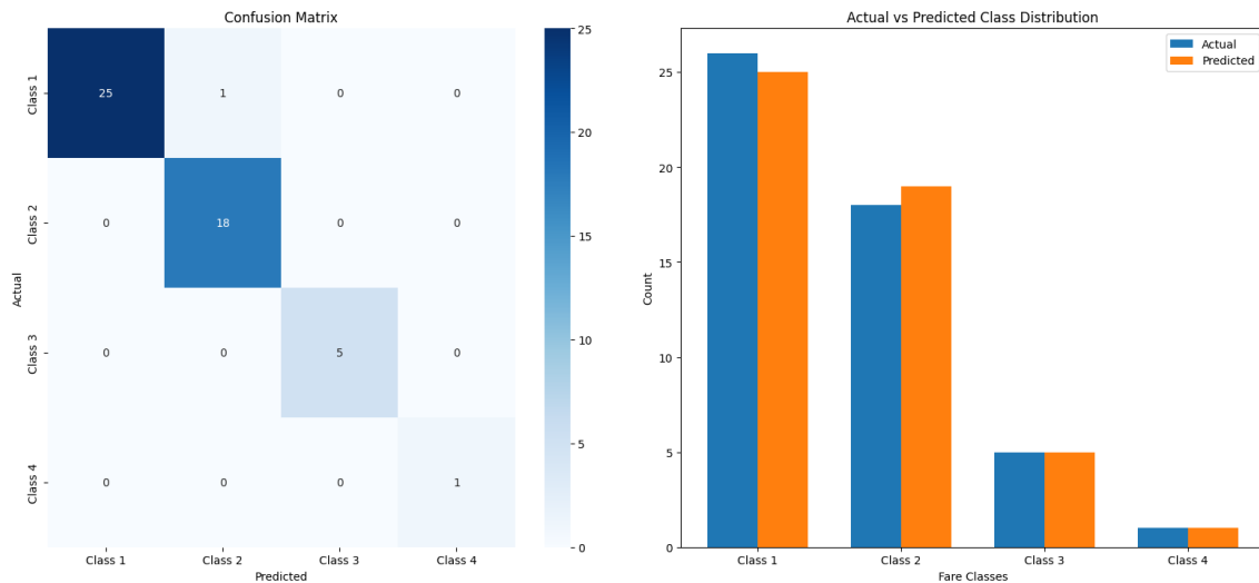
Fig. 3. kNN Classification
