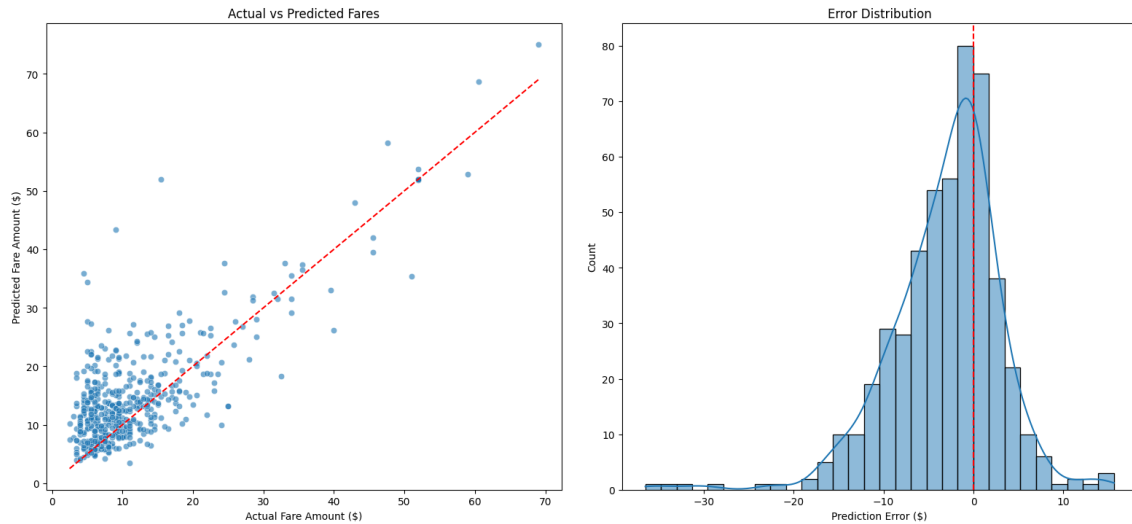
Fig. 2. kNN Regression
